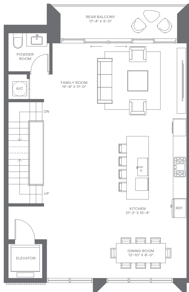
LEVEL 2
